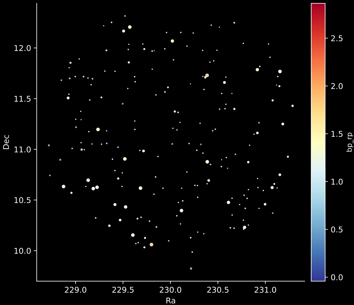
APOGEE DR17 Field: [K2_C5_215+29_btx] Stars: 198
