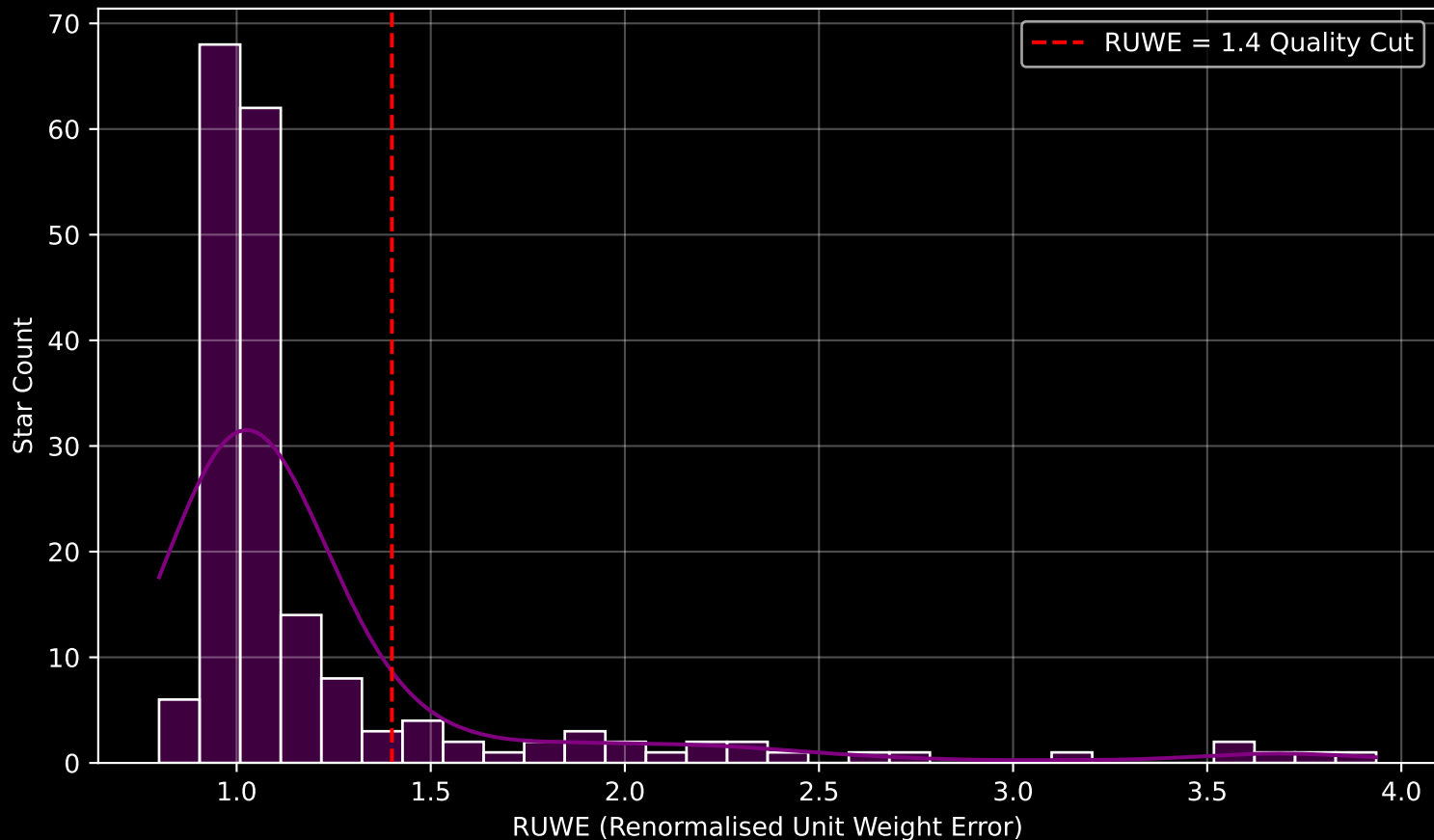
GAPOGEE DR17 Field [K2_C5_215+29_btx] RUWE Distribution (n= 189)
