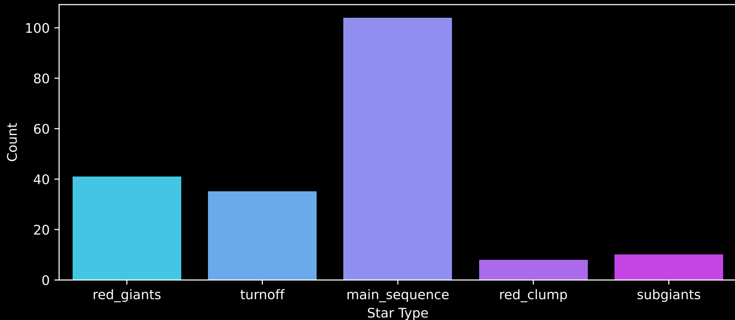
APOGEE DR17 Field: [K2_C5_215+29_btx] Count plot of Star Type
