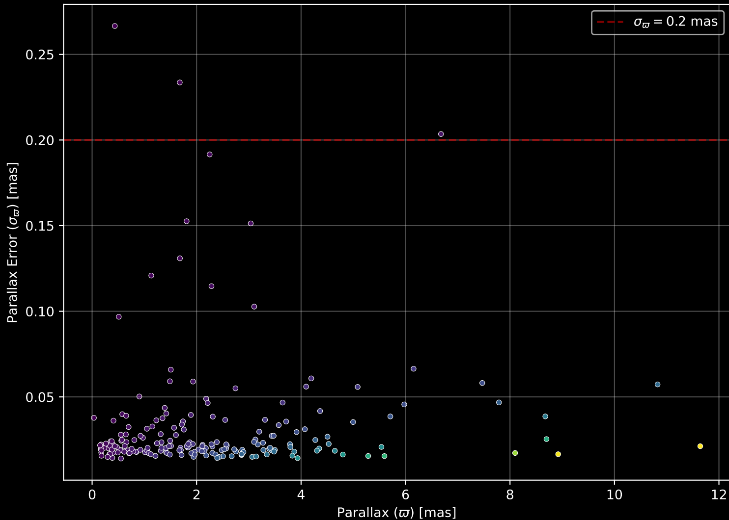
APOGEE DR17 Field: [K2_C5_215+29_btx] Parallax Quality (n= 198)
