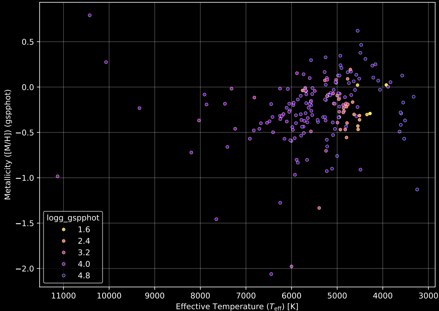
APOGEE DR17 Field: [K2_C5_215+29_btx] Stellar Population Parameters (n= 198)
