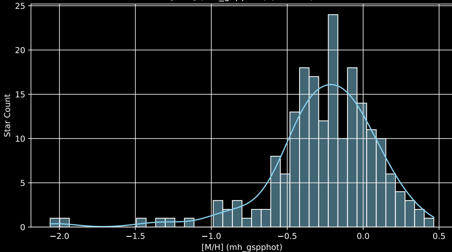
APOGEE DR17 Field: [K2_C5_215+29_btx [M/H] (mh_gspphot) (n= 196)
