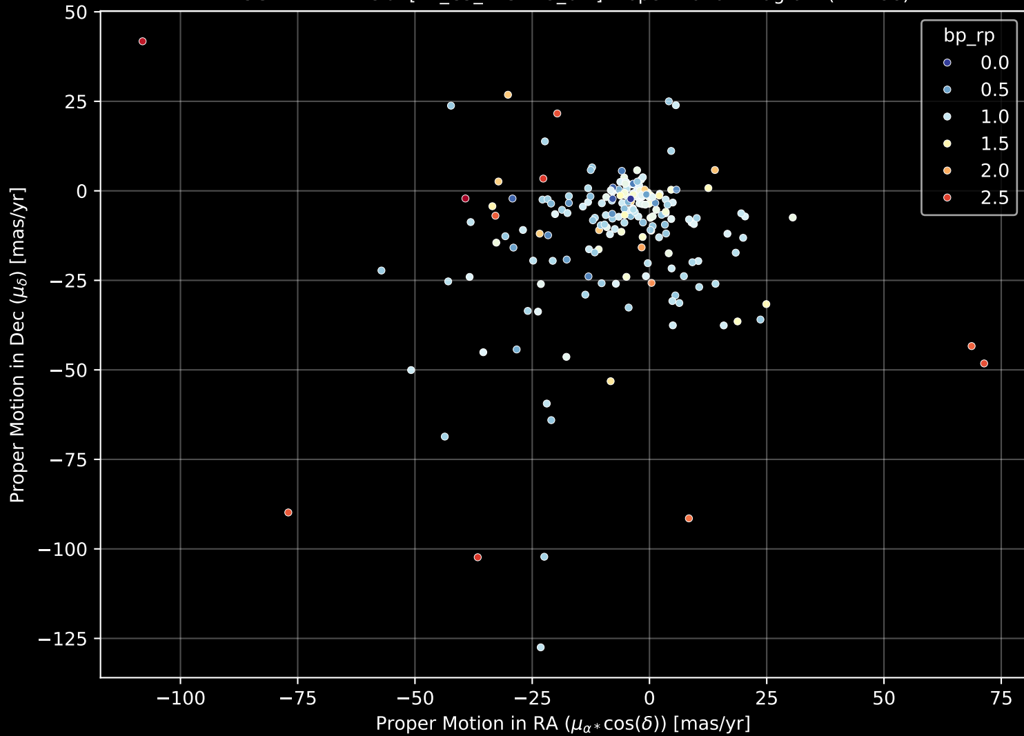
APOGEE DR17 Field: [K2_C5_215+29_btx] Proper Motion Diagram (n= 198)
